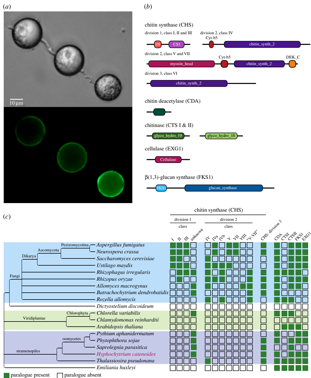
Figure 6 Comparative genomic analysis of gene families that function in cell-wall synthesis. (a) Micrographs showing the wheat germ agglutinin fluorescent staining of a chitin cell wall on Hyphochytrium structures. (b) The domain architecture of eight proteins that function in cell-wall synthesis. (c) The taxon distribution of putative gene families associated with cell-wall synthesis across a representative set of taxa including the Pseudofungi.
